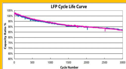
Curve of cycle life
