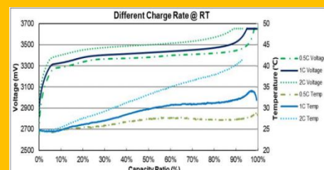
Curve of different charge rate
