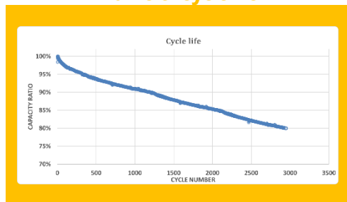
Curve of cycle life
