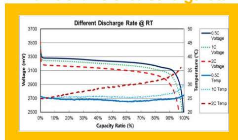
Curve of different discharge rate
