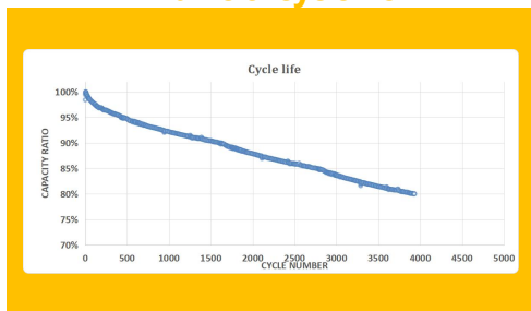
Curve of cycle life
