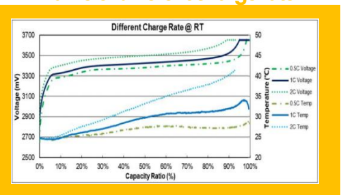
Curve of different charge rate
